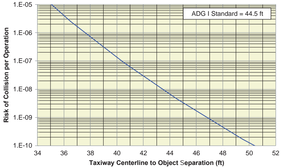
Figure AA-8. Collision risk associated with taxiway to object separation for ADG I.
