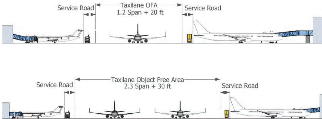
Figure 4. Wingtip clearance for taxilanes.
