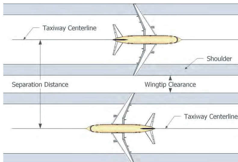
Figure 1. Wingtip clearance, parallel taxiways.
