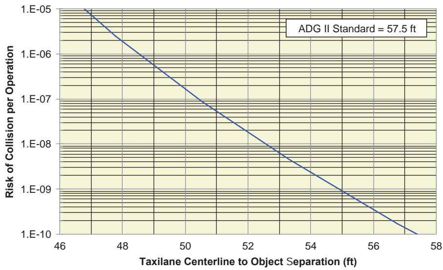
Figure AA-23. Collision risk associated with taxilane to object separation for ADG II.
