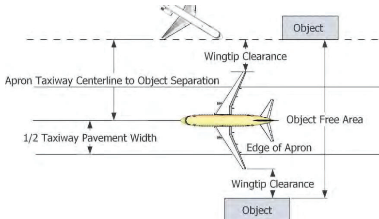
Figure 3. Wingtip clearance for taxilanes.
