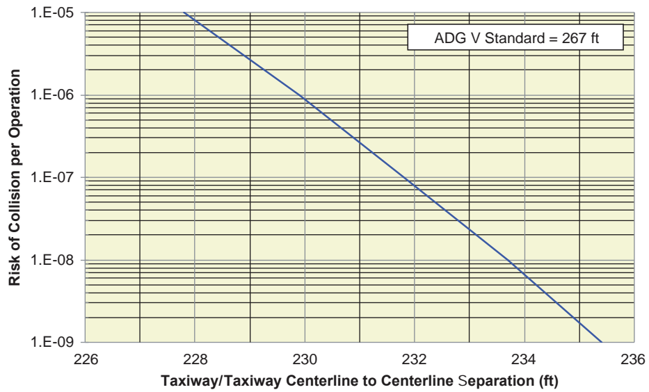
Figure AA-5. Collision risk associated with taxiway centerline separation for ADG V.
