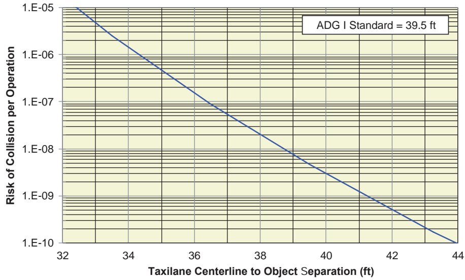
Figure AA-22. Collision risk associated with taxilane to object separation for ADG I.
