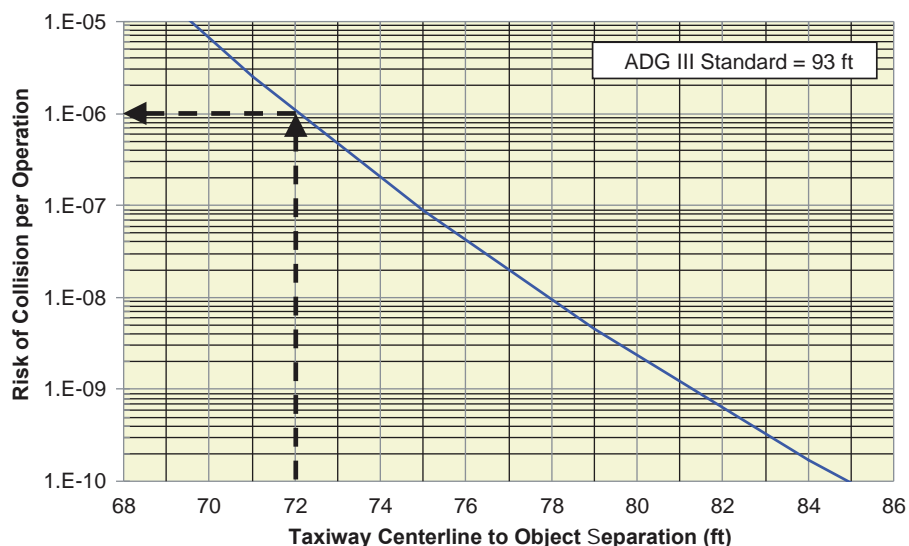
Figure A-7. Example of analysis for taxiway/object separation (ADG III).
