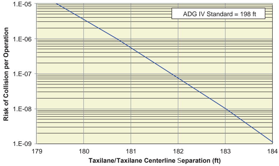
Figure AA-18. Collision risk associated with taxilane to object separation for ADG IV.
