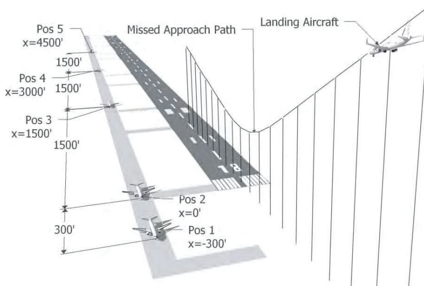
Figure 17. Perspective view of CRM run experiment (not to scale).
