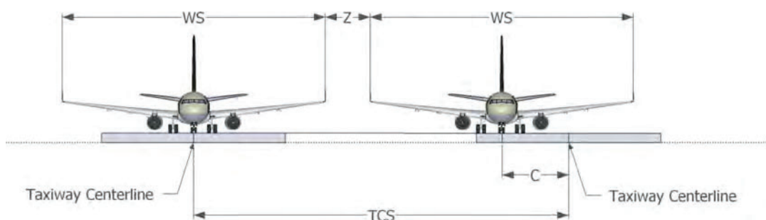
Figure 6. Parallel taxiway separation geometry.
