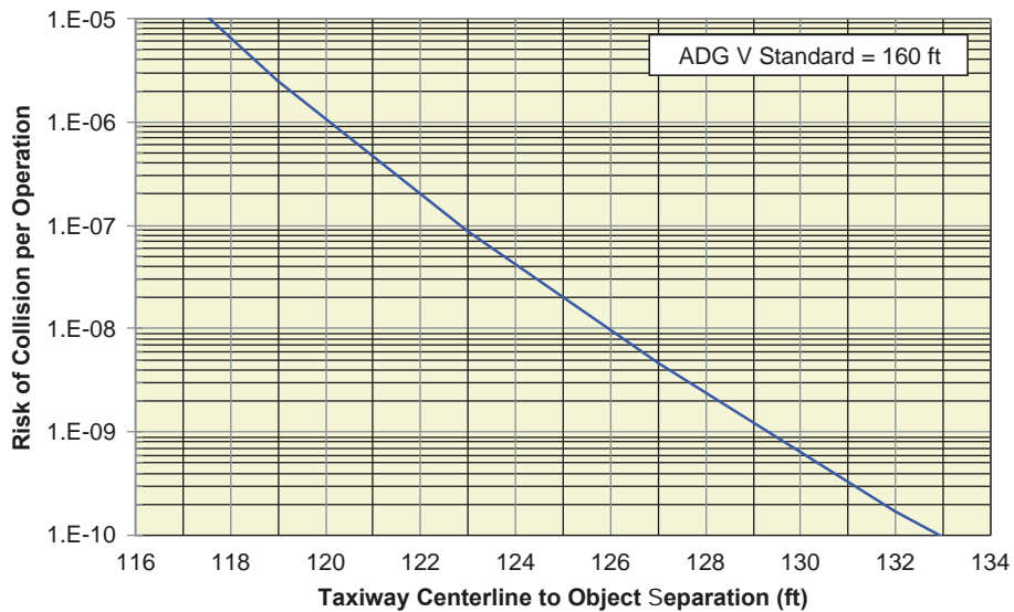
Figure AA-12. Collision risk associated with taxiway to object separation for ADG V.
