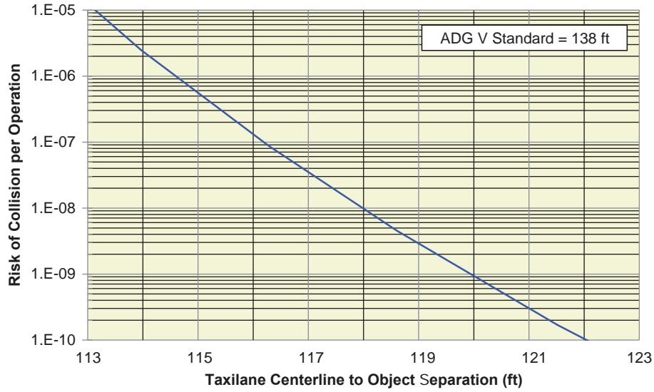
Figure AA-26. Collision risk associated with taxilane to object separation for ADG V.
