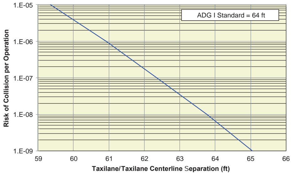
Figure AA-15. Collision risk associated with taxilane to object separation for ADG I.
