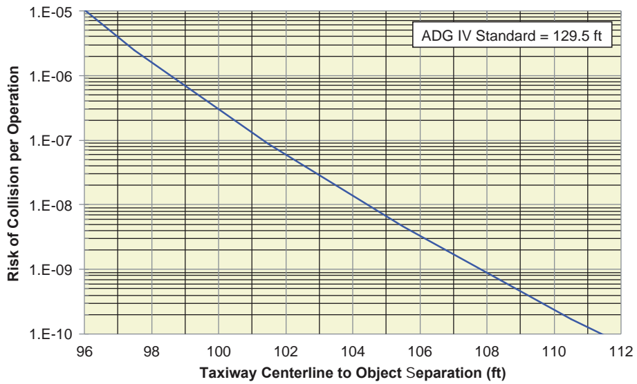
Figure AA-11. Collision risk associated with taxiway to object separation for ADG IV.
