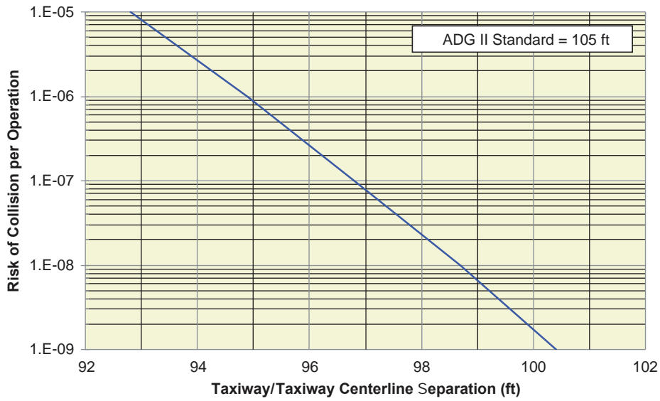
Figure AA-2. Collision risk associated with taxiway centerline separation for ADG II.
