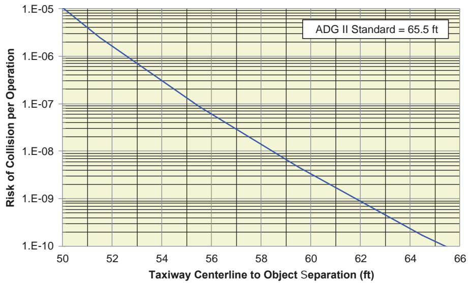
Figure AA-9. Collision risk associated with taxiway to object separation for ADG II.
