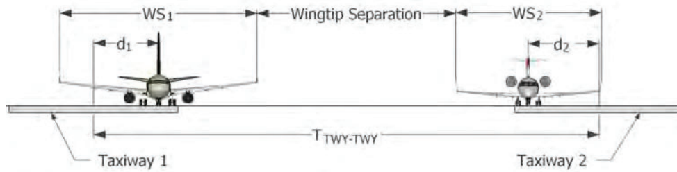
Figure 10. Taxiway/taxiway separation.
