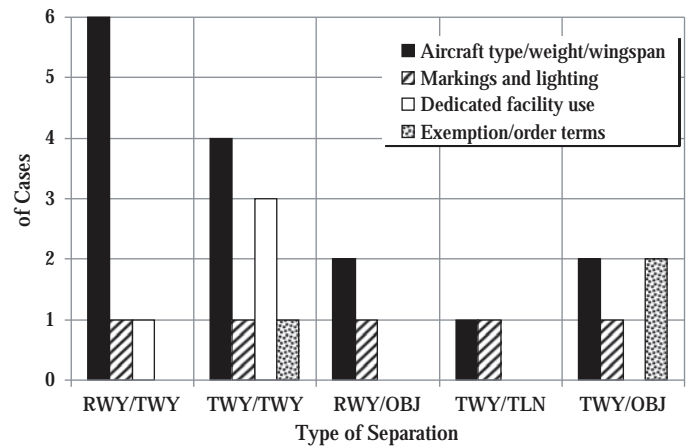
Figure 24. Most common restrictions for MOS of airfield separations.
