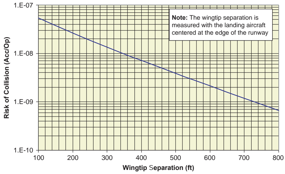
Figure AA-54. Takeoff veer-off collision risk based on wingtip clearance—any ADG.
