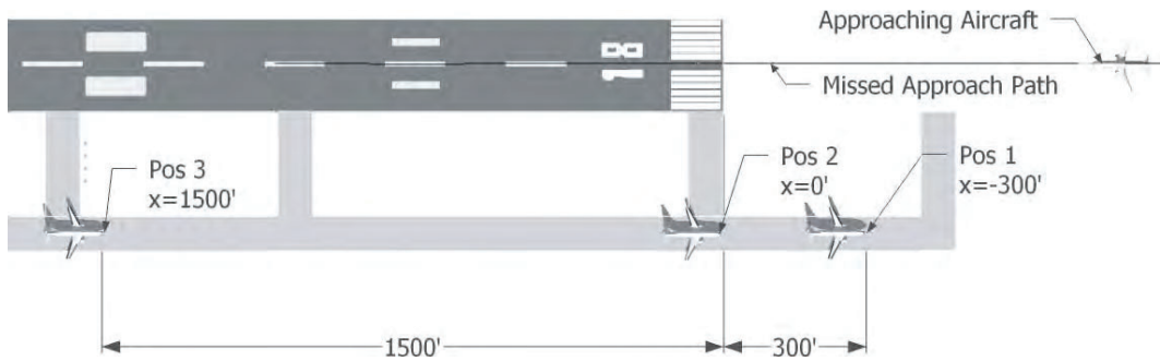
Figure 16. Plan view of CRM run experiment.
