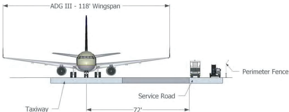
Figure A-6. Example of analysis for taxiway/object separation.
