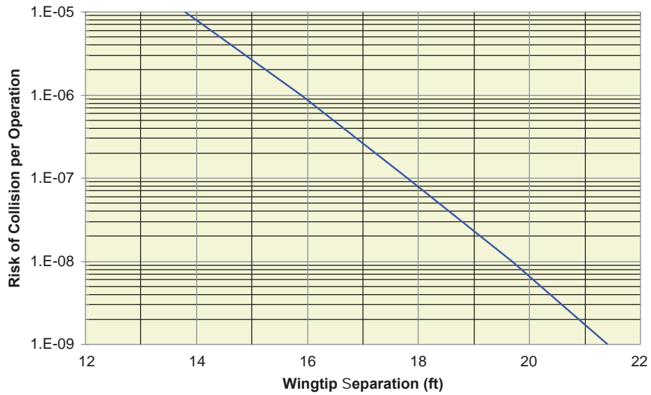
Figure AA-7. Collision risk associated with wingtip separation distance (Any ADG).
