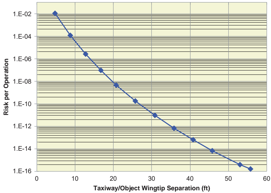
Figure 13. Taxiway/object collision probability based on wingtip separation.
