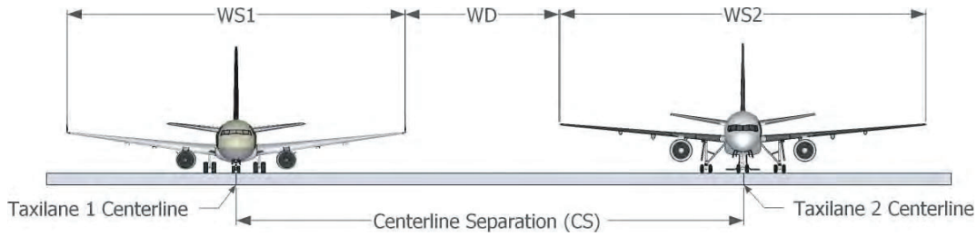
Figure A-8. Example of taxilane/taxilane separation analysis for specific aircraft.
