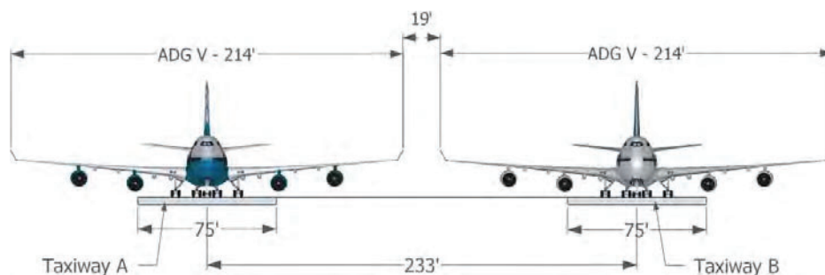
Figure A-3. Example of analysis for taxiway/taxiway separation.
