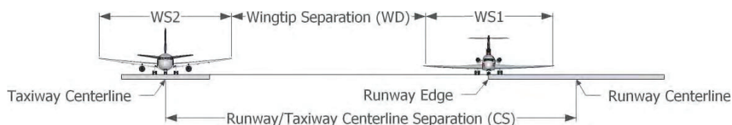
Figure A-11. Typical runway/taxiway scenario for runway veer-off incidents.
