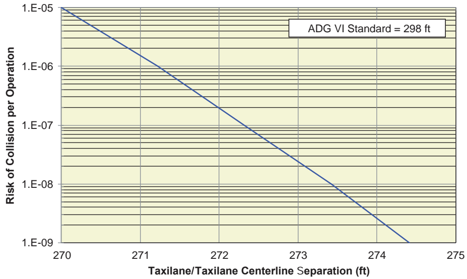
Figure AA-20. Collision risk associated with taxilane to object separation for ADG VI.
