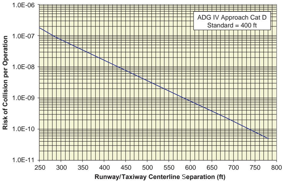
Figure AA-35. Missed approach collision risk for ADG IV Cat I.
