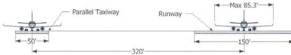
Figure A-13. Example of Runway/Taxiway Separation.
