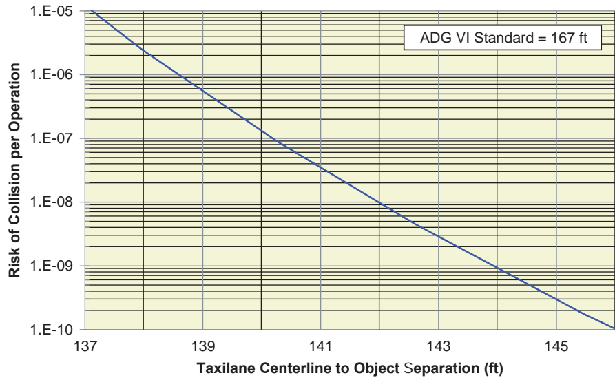
Figure AA-27. Collision risk associated with taxilane to object separation for ADG VI.
