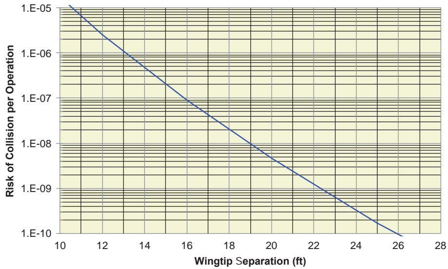
Figure AA-14. Collision risk associated with taxiway wingtip to object clearance (any ADG).
