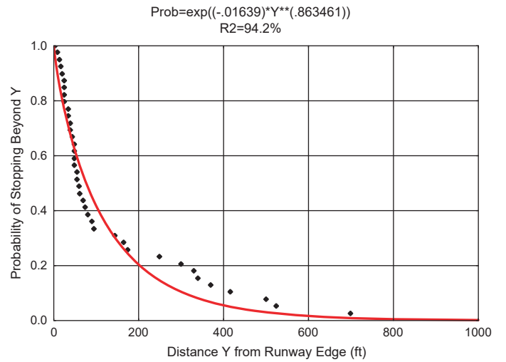
Figure 22. Location model for takeoff veer-off.
