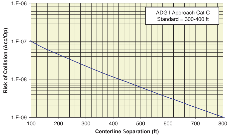
Figure AA-48. Takeoff veer-off collision risk for ADG I.
