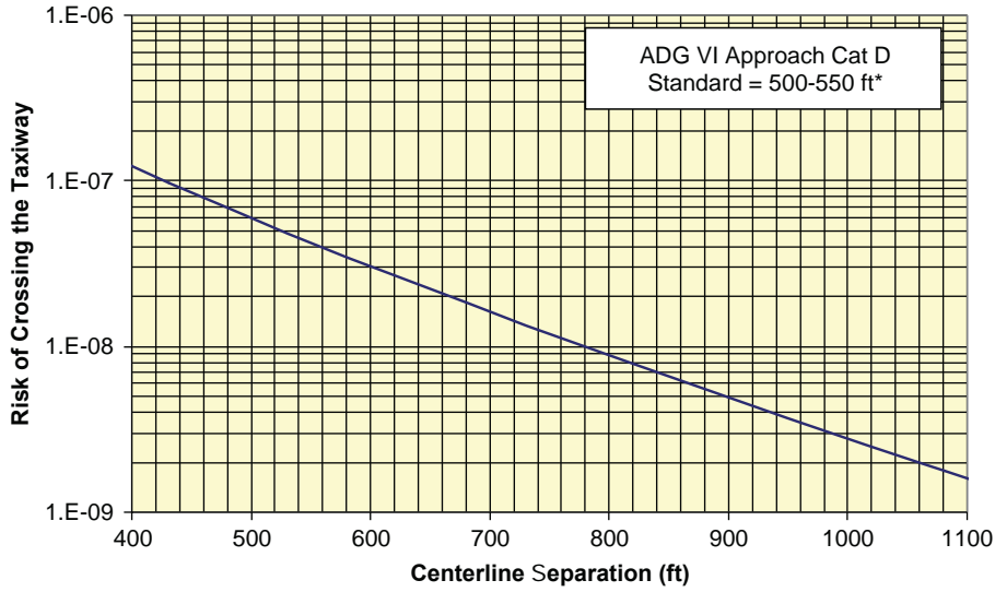
Figure AA-46. Landing veer-off collision risk for ADG VI.
