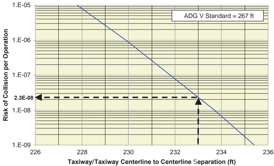
Figure A-4. Example of analysis of taxiway/taxiway separation (ADG V).
