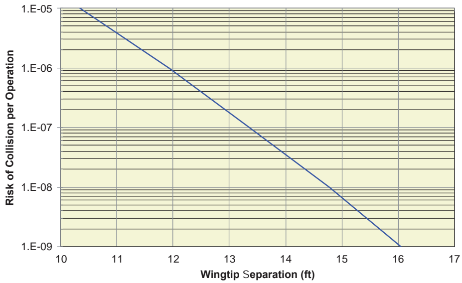
Figure AA-21. Collision risk associated with taxilane wingtip separation distance (any ADG).
