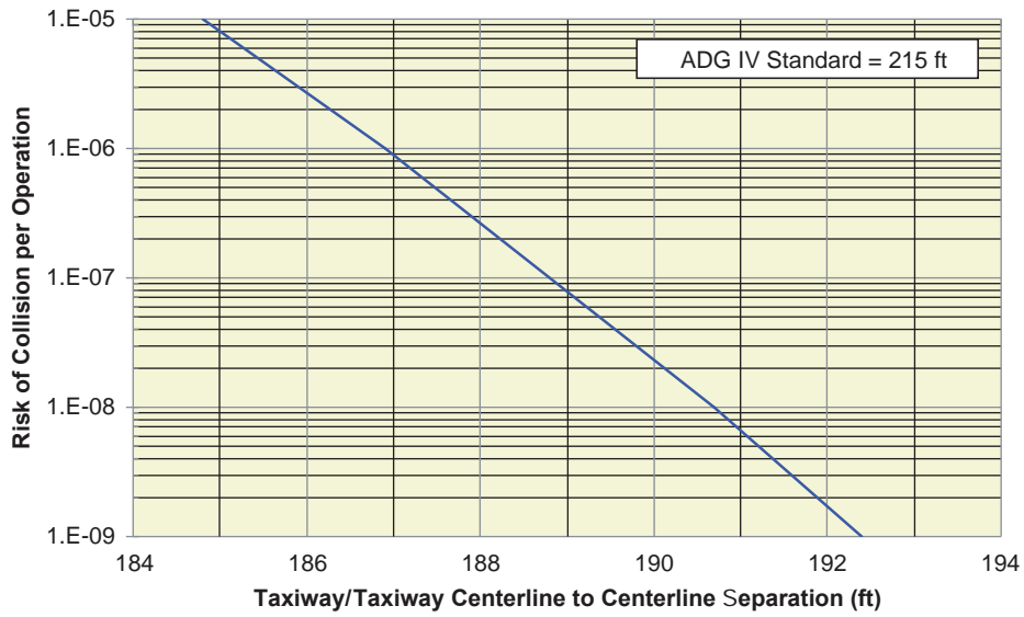
Figure AA-4. Collision risk associated with taxiway centerline separation for ADG IV.
