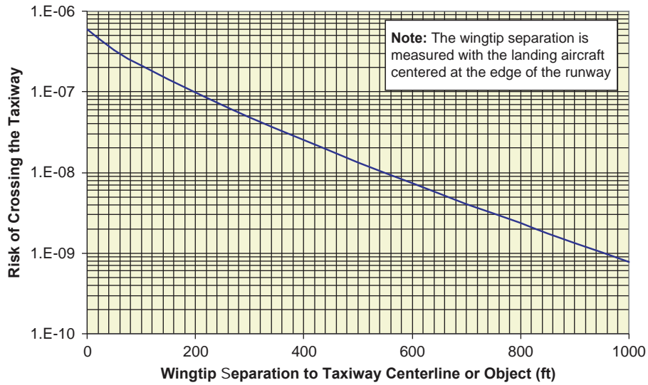
Figure AA-47. Landing veer-off collision risk based on wingtip clearance—any ADG.
