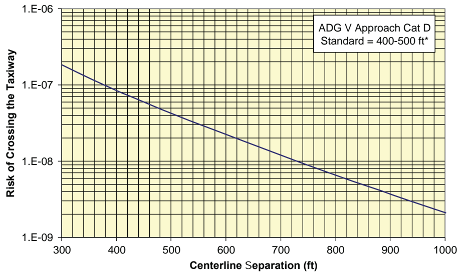
Figure AA-45. Landing veer-off collision risk for ADG V.
