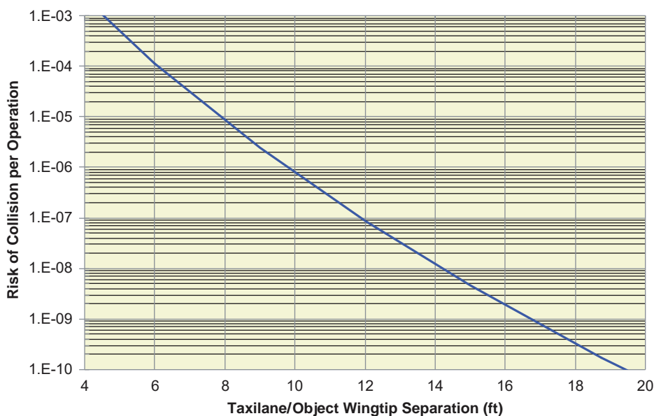
Figure 15. Taxilane/object collision risk based on wingtip separation.
