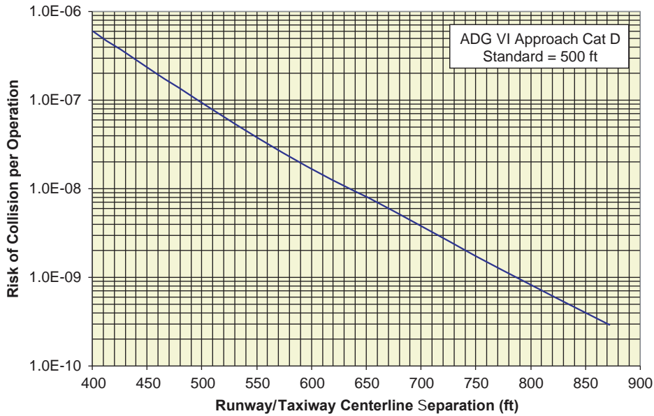
Figure AA-39. Missed approach collision risk for ADG VI Cat I.
