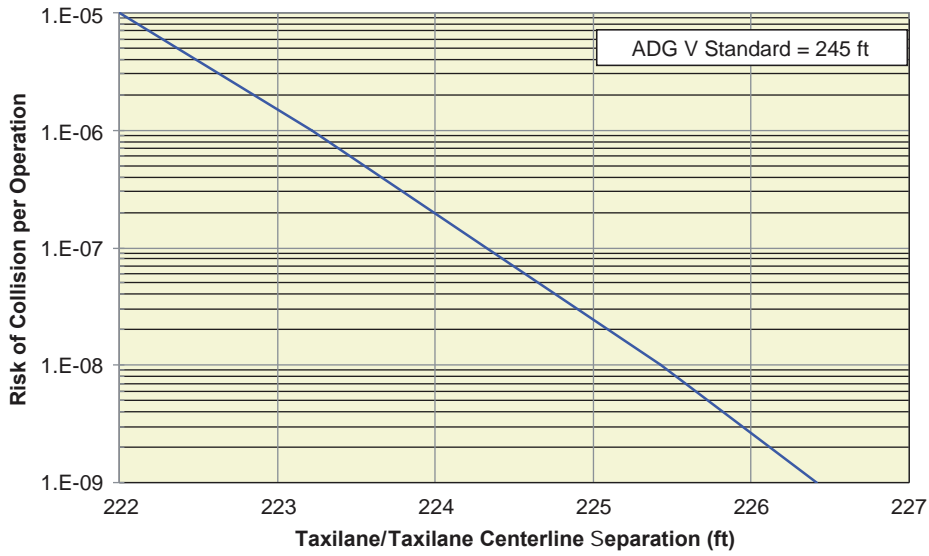
Figure AA-19. Collision risk associated with taxilane to object separation for ADG V.
