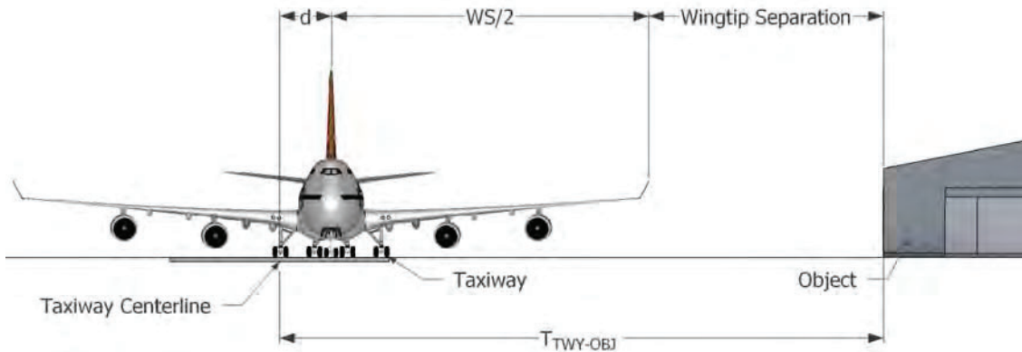
Figure 11. Taxiway/object separation.
