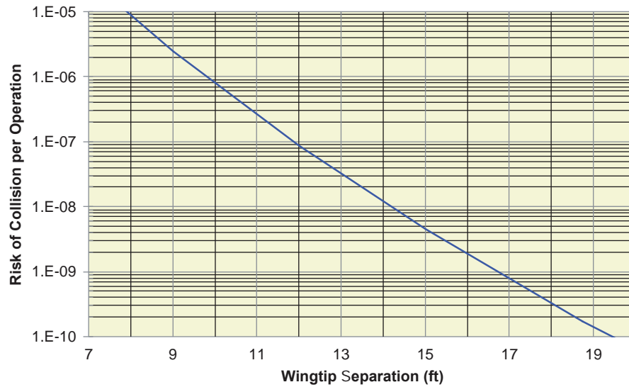
Figure AA-28. Collision risk associated with taxilane wingtip to object clearance—any ADG.
