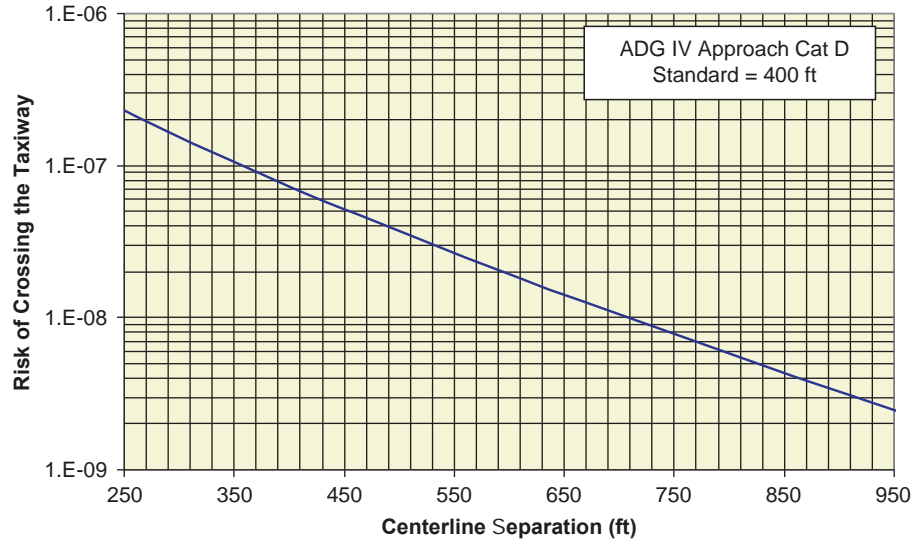
Figure AA-44. Landing veer-off collision risk for ADG IV.
