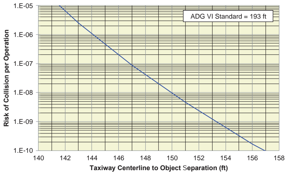
Figure AA-13. Collision risk associated with taxiway to object separation for ADG VI.
