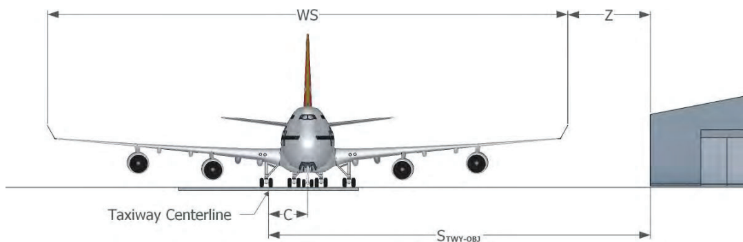
Figure 7. Taxiway/apron taxiway-to-object geometry.
