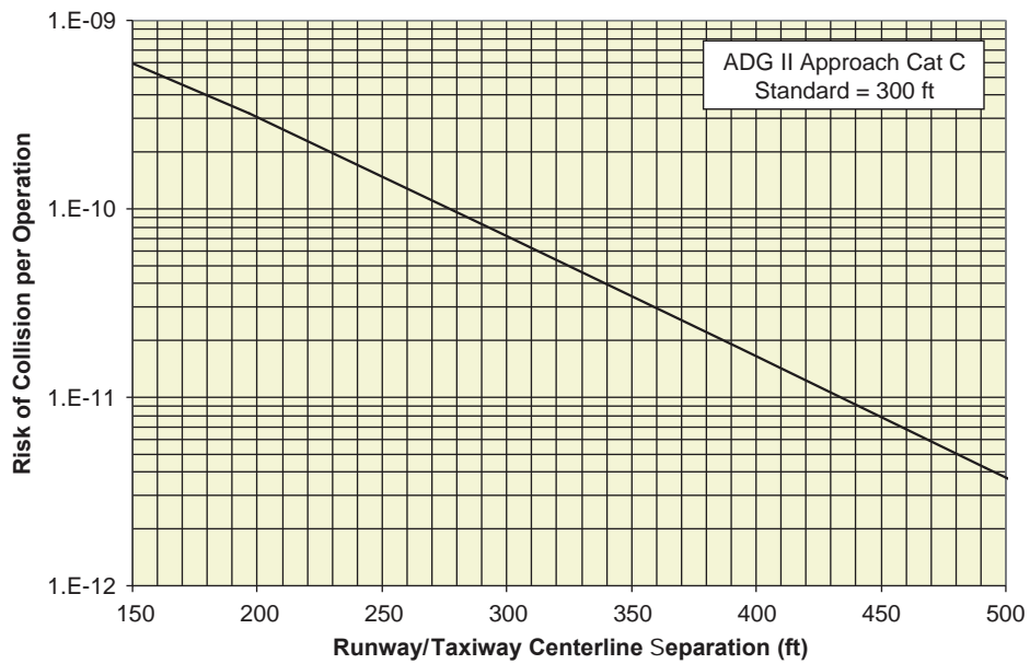
Figure AA-31. Missed approach collision risk for ADG II Cat I.
