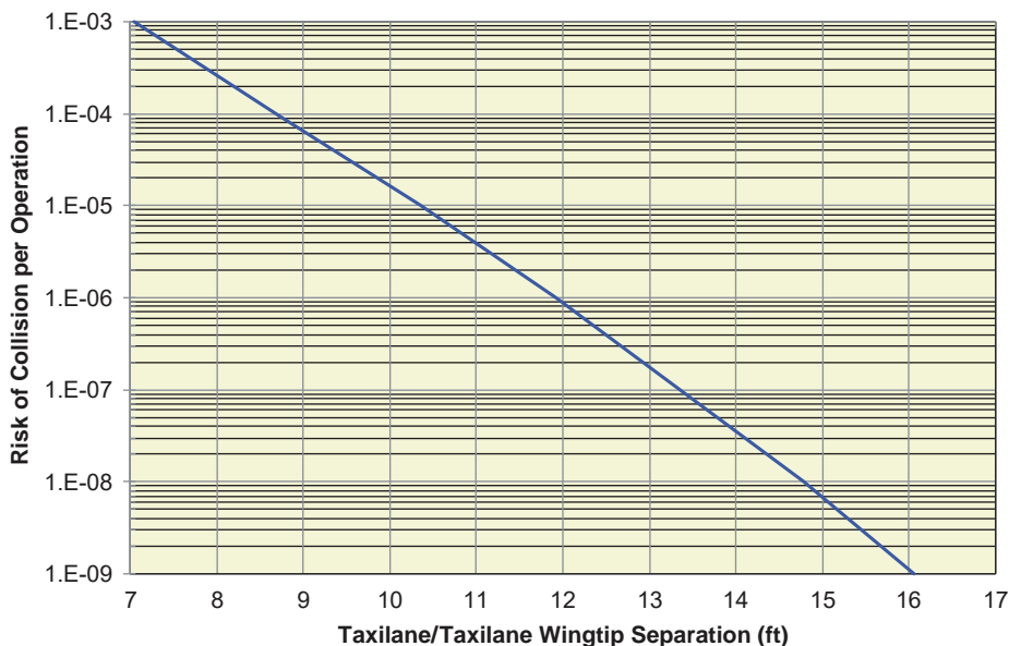
Figure 14. Taxilane/taxilane collision probability based on wingtip separation.
