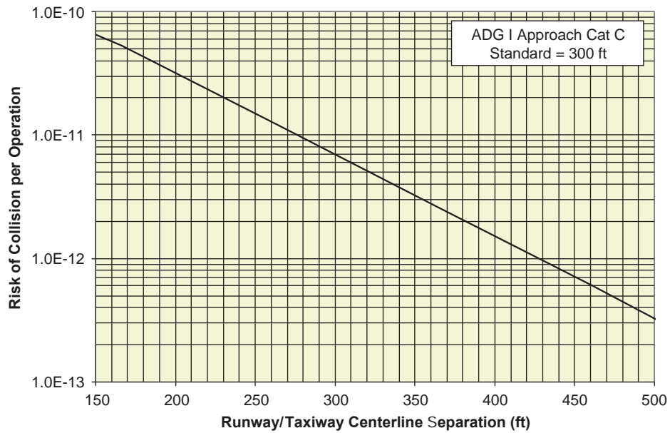
Figure AA-29. Missed approach collision risk for ADG I Cat I.
