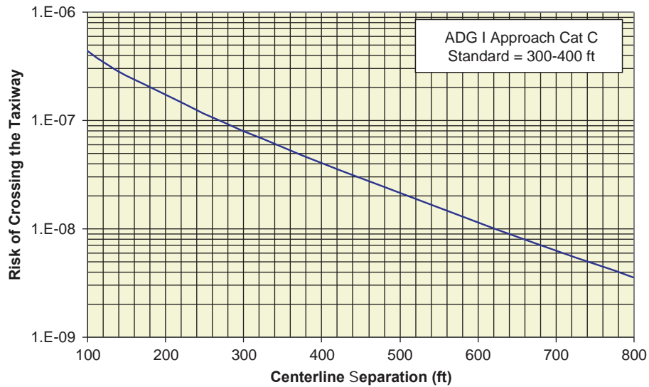
Figure AA-41. Landing veer-off collision risk for ADG I.
