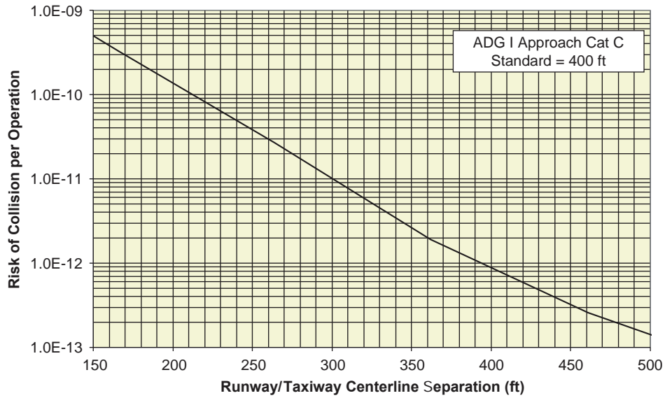
Figure AA-30. Missed approach collision risk for ADG I Cat II.
