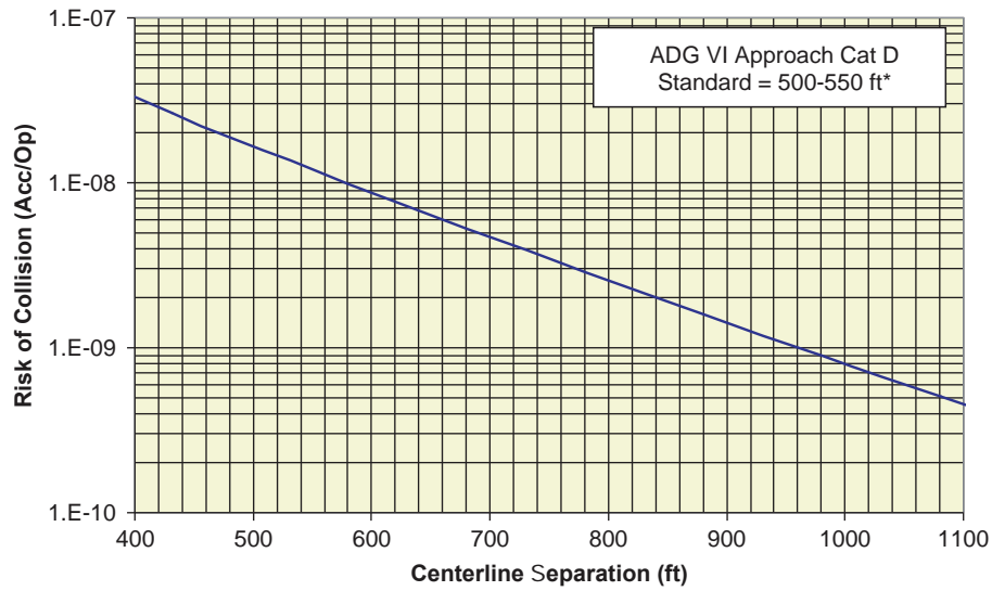
Figure AA-53. Takeoff veer-off collision risk for ADG VI.
