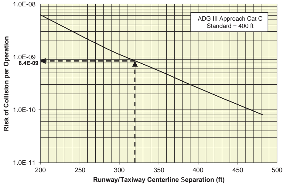
Figure A-14. Estimating airborne risk of runway/taxiway separation (ADG III-CAT I).
