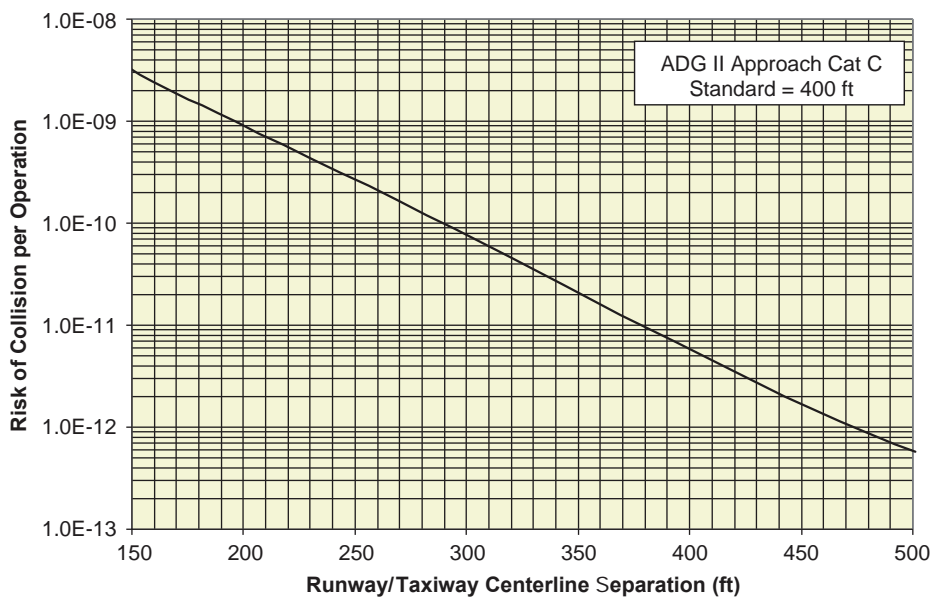
Figure AA-32. Missed approach collision risk for ADG II Cat II.
