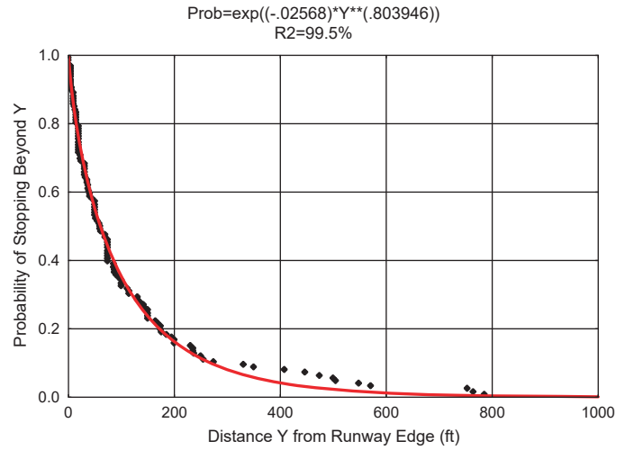
Figure 21. Location model for landing veer-off.
