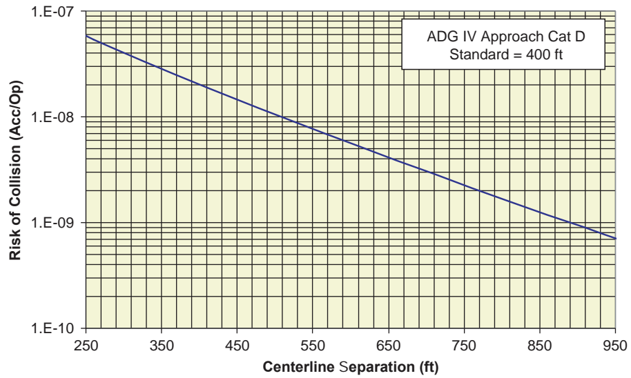
Figure AA-51. Takeoff veer-off collision risk for ADG IV.
