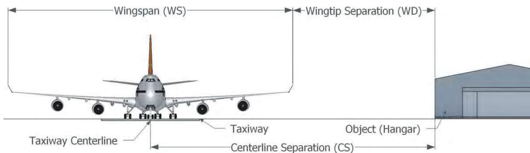
Figure A-5. Example of taxiway/object separation analysis for specific aircraft.
