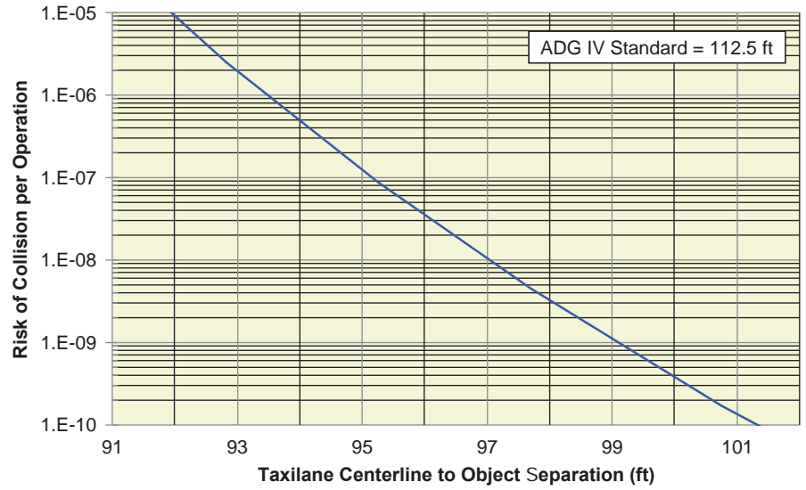
Figure AA-25. Collision risk associated with taxilane to object separation for ADG IV.
