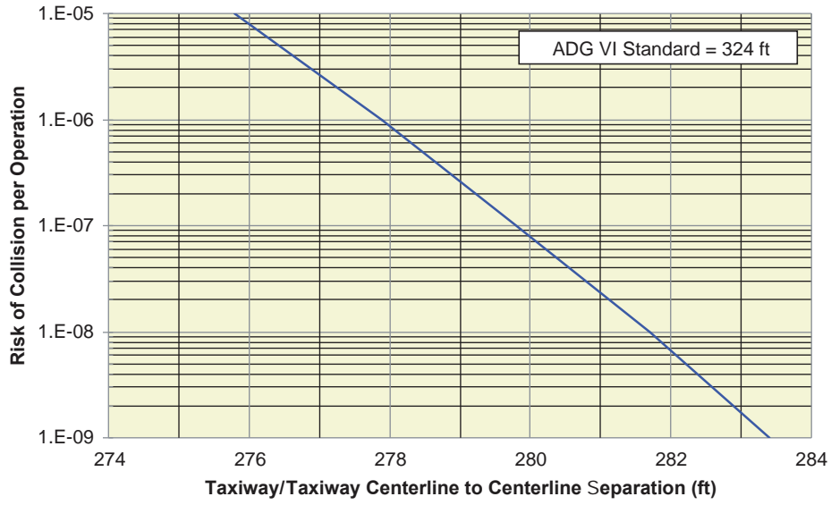
Figure AA-6. Collision risk associated with taxiway centerline separation for ADG VI.
