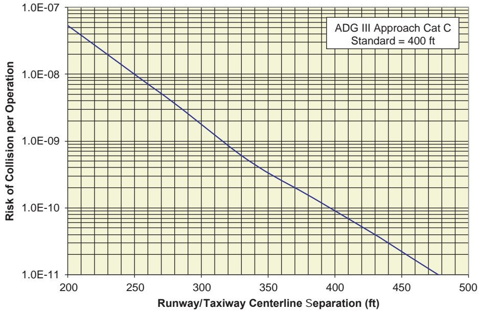
Figure AA-34. Missed approach collision risk for ADG III Cat II.
