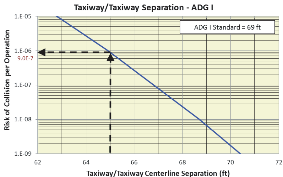
Exhibit AA-1. Example illustrating use of plots.
