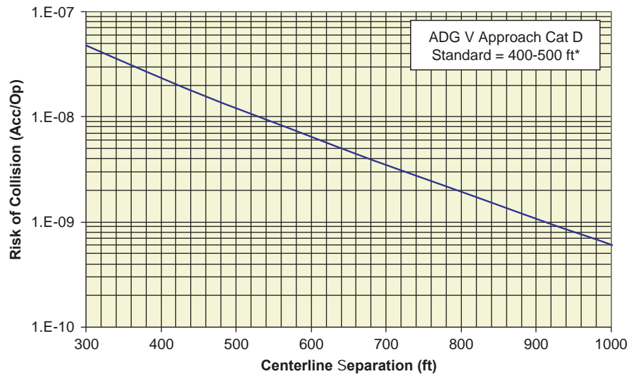
Figure AA-52. Takeoff veer-off collision risk for ADG V.
