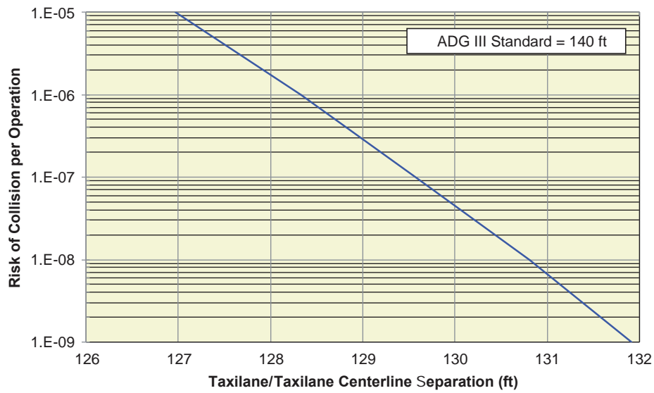
Figure AA-17. Collision risk associated with taxilane to object separation for ADG III.
