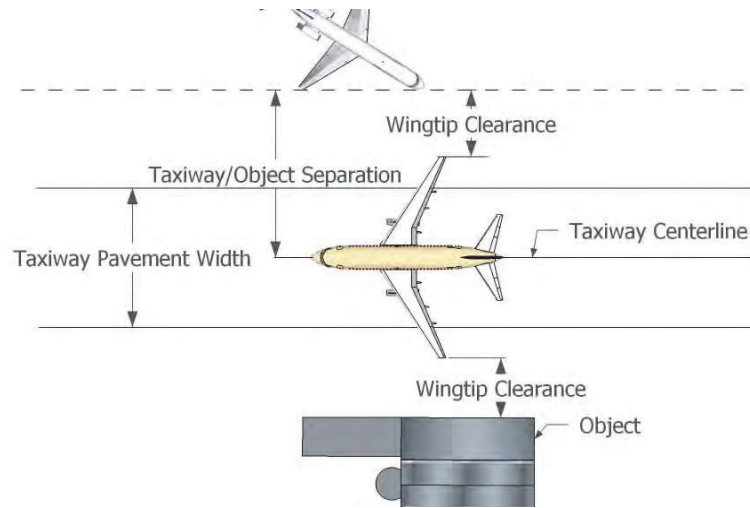
Figure 2. Wingtip clearance from taxiway.
