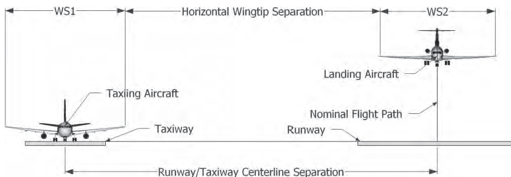
Figure A-10. Example of runway/taxiway separation analysis.
