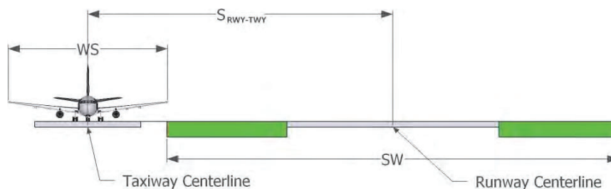
Figure 5. Runway/parallel taxiway separation distance.
