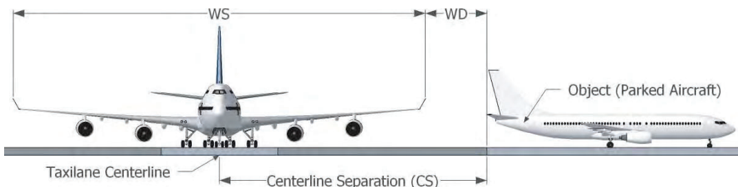
Figure A-9. Example of taxiway/object separation analysis for specific aircraft.
