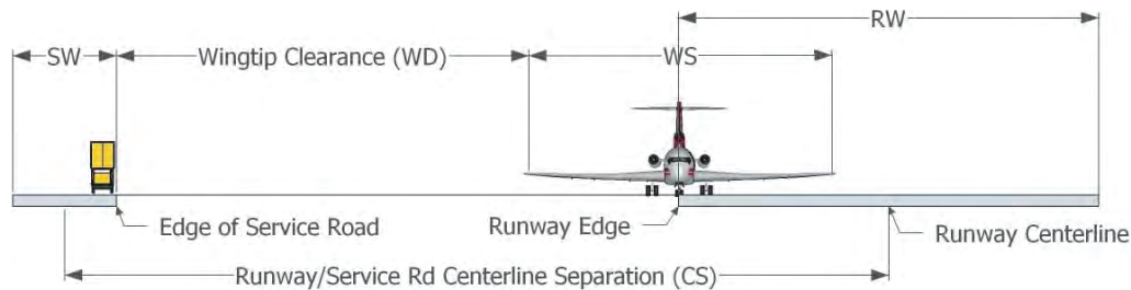
Figure A-12. Typical runway/object scenario for runway veer-off incidents.
