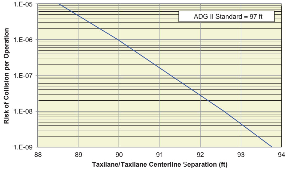
Figure AA-16. Collision risk associated with taxilane to object separation for ADG II.
