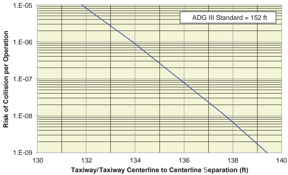
Figure AA-3. Collision risk associated with taxiway centerline separation for ADG III.
