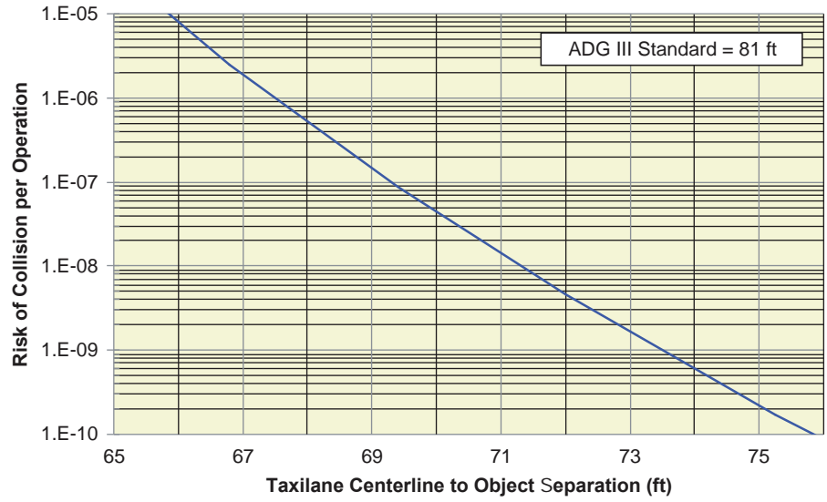
Figure AA-24. Collision risk associated with taxilane to object separation for ADG III.
