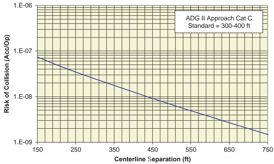
Figure AA-49. Takeoff veer-off collision risk for ADG II.
