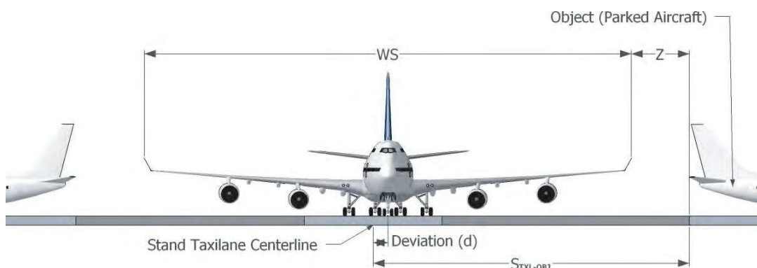
Figure 8. Aircraft stand taxilane-to-object geometry.
