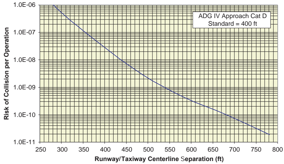
Figure AA-36. Missed approach collision risk for ADG IV Cat II.
