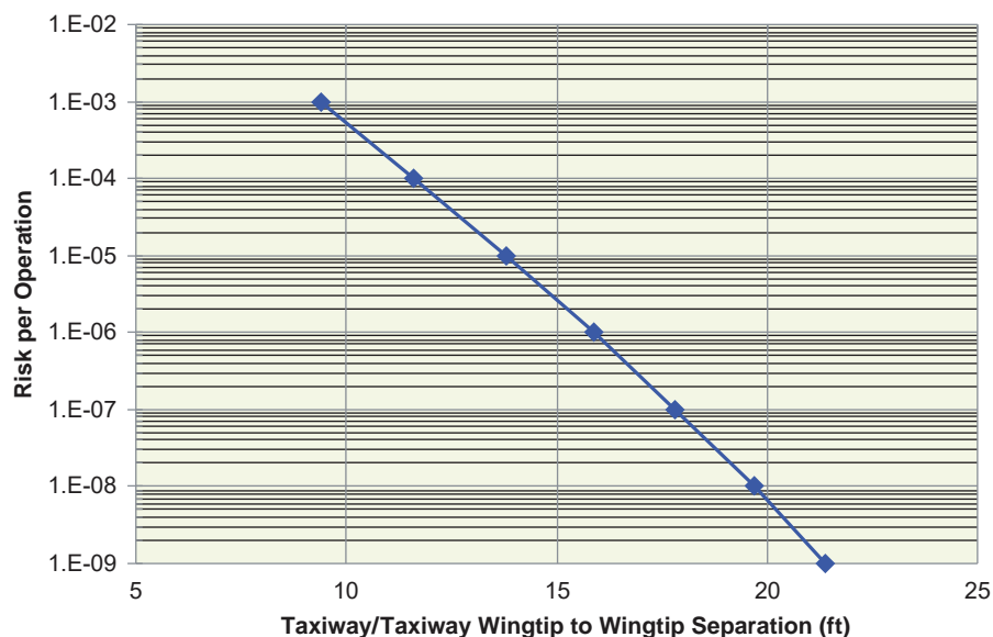
Figure 12. Taxiway/taxiway collision risk.
