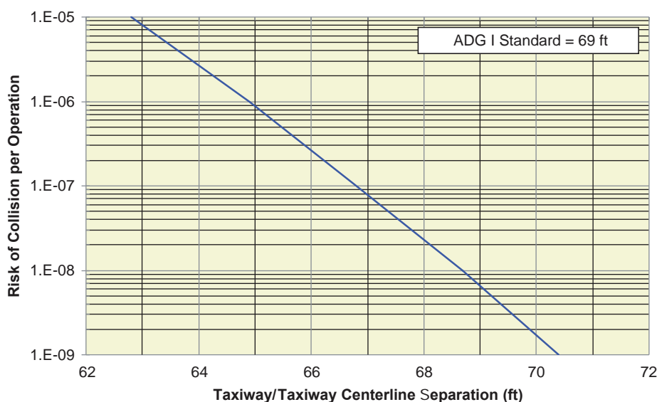
Figure AA-1. Collision risk associated with taxiway centerline separation for ADG I.
