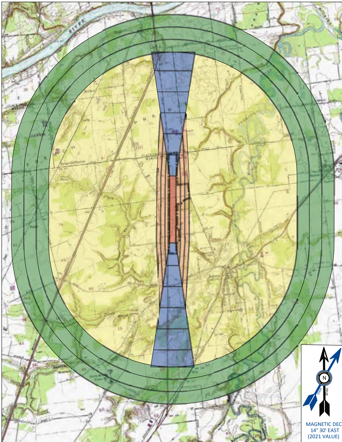
FIGURE 2-10: PART 77 AIRSPACE
