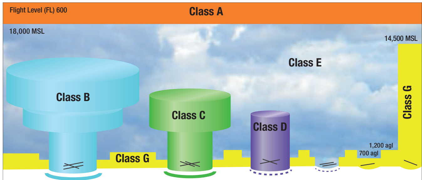
FIGURE 2-11: AIRSPACE CLASSIFICATIONS
