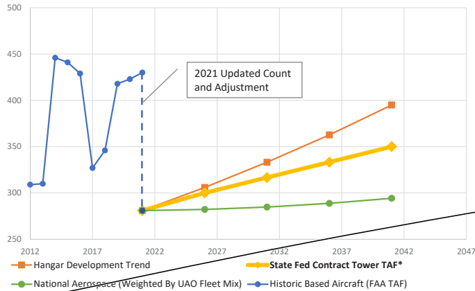
FIGURE 3-4: BASED AIRCRAFT FORECASTS
