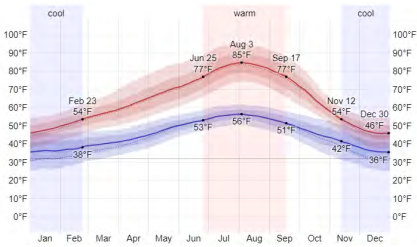
FIGURE 2-4: ANNUAL TEMPERATURES
