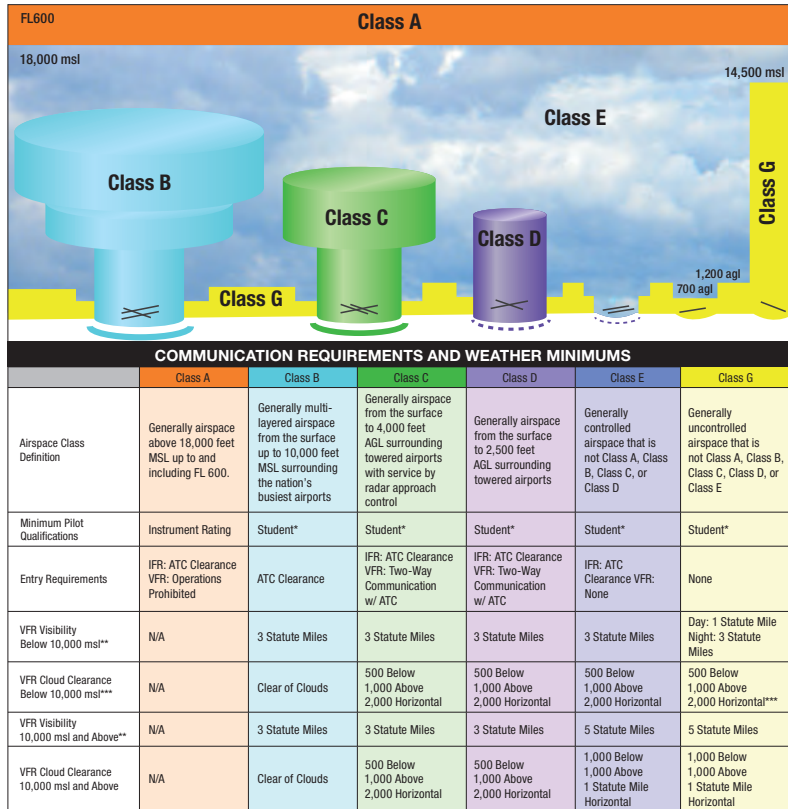
FIGURE 2-11: AIRSPACE CLASSIFICATIONS
