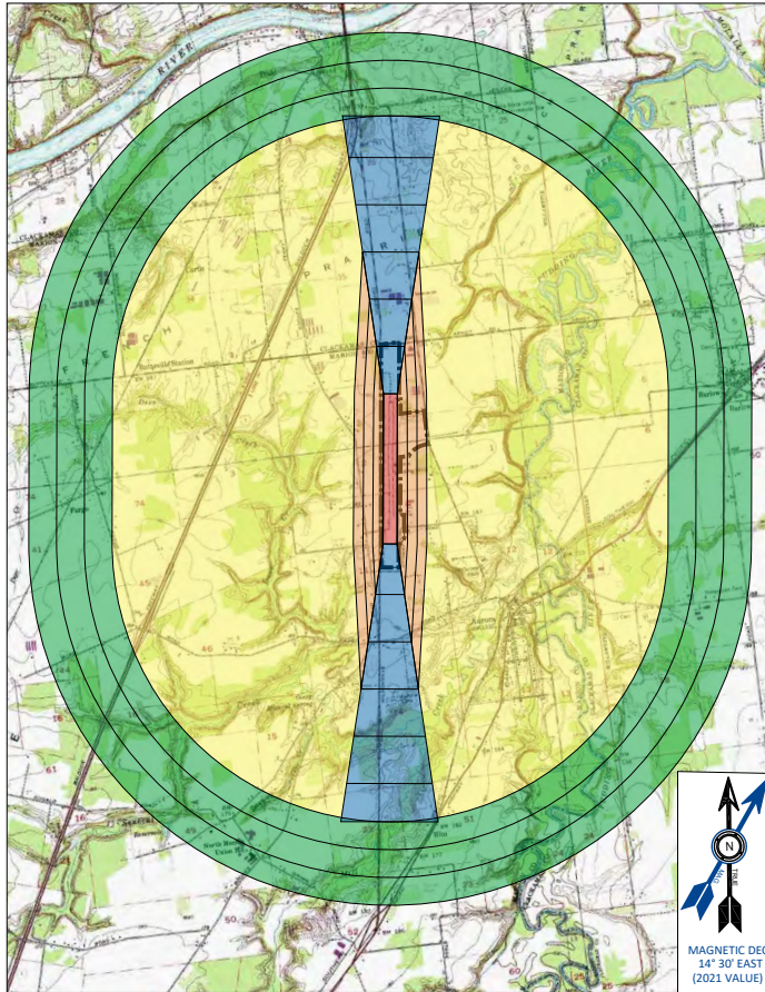
FIGURE 2-10: PART 77 AIRSPACE
