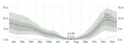
FIGURE 2-5: ANNUAL RAINFALL
