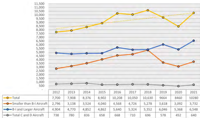
FIGURE 2-3: TFMS IFR OPERATIONS DATA
