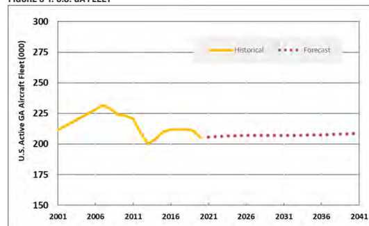
FIGURE 3-1: U.S. GA FLEET
