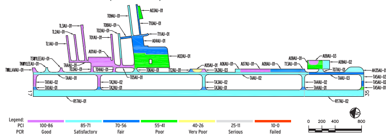
FIGURE 2-14: PAVEMENT CONDITIONS (2018 INSPECTION)
