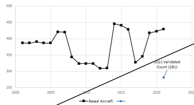
FIGURE 3-2: HISTORICAL TAF – BASED AIRCRAFT
