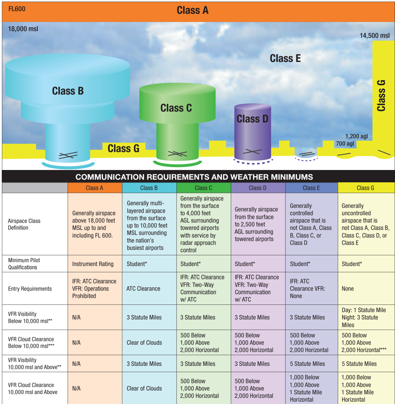
FIGURE 2-11: AIRSPACE CLASSIFICATIONS
