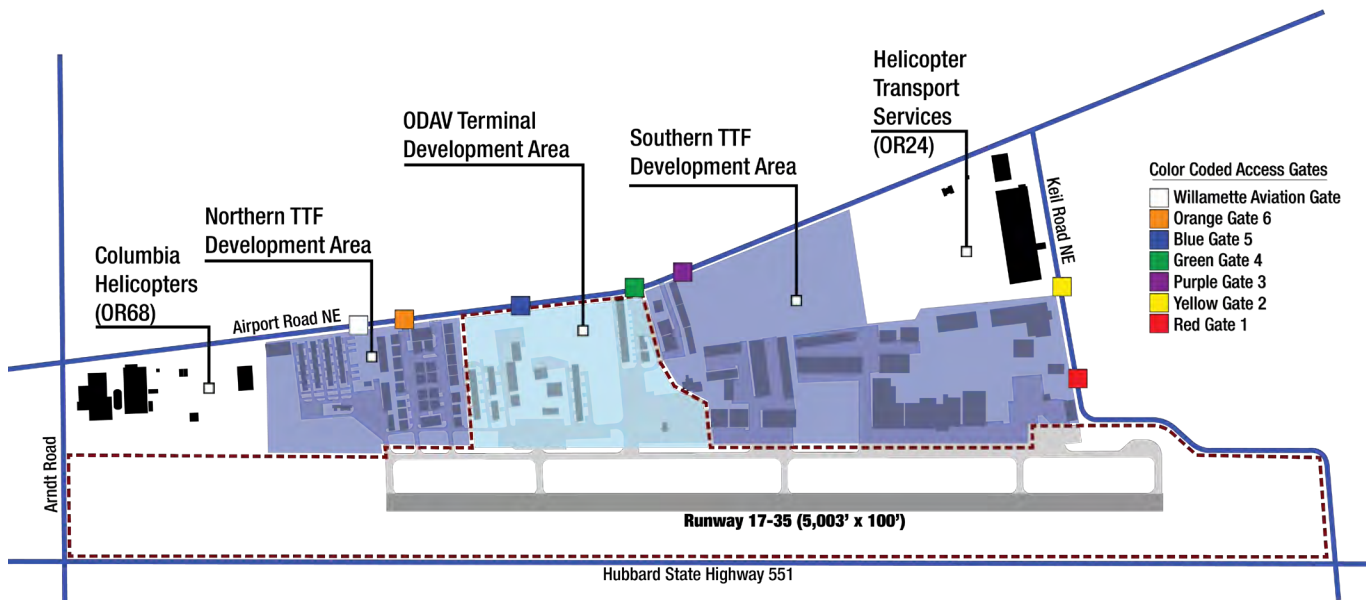
FIGURE 2-16: AURORA STATE AIRPORT DEVELOPMENT AREAS
