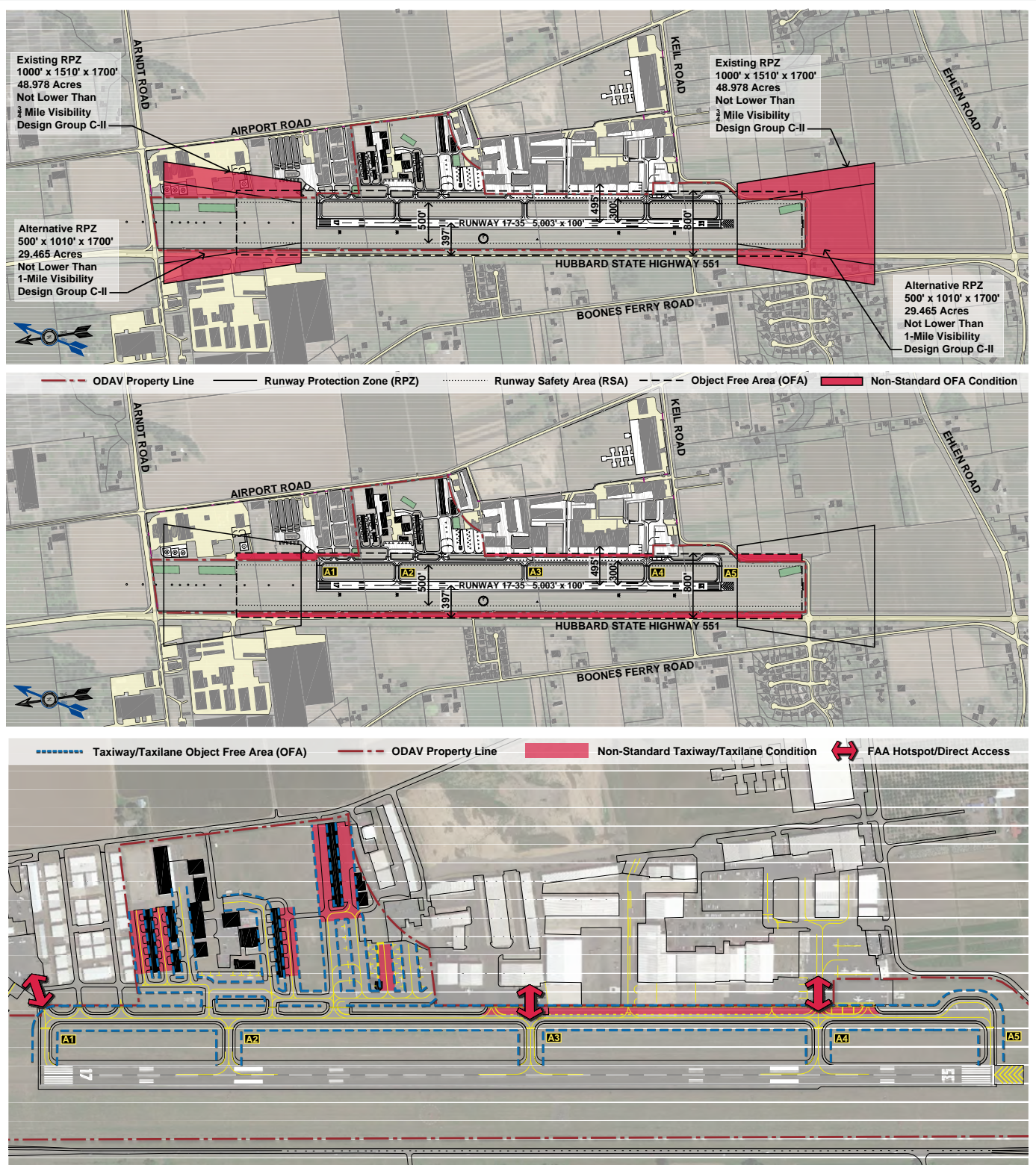
FIGURE 2-15: NON-STANDARD CONDITIONS
