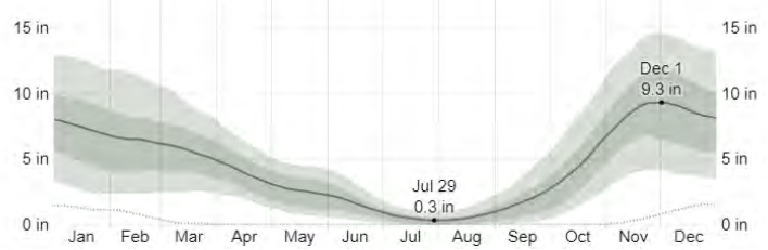
FIGURE 2-5: ANNUAL RAINFALL
